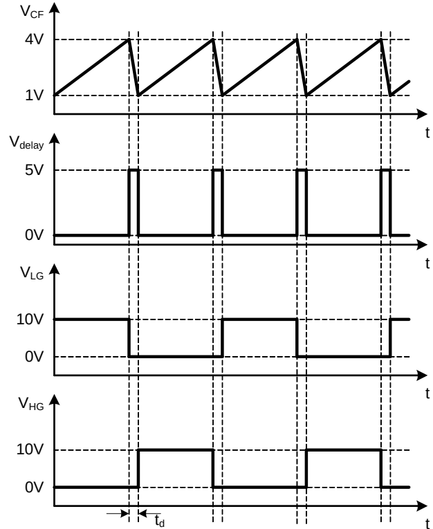
Figure 4 Oscillator waveforms
