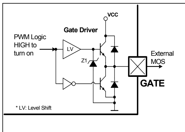
Figure 23 Gate Driver
