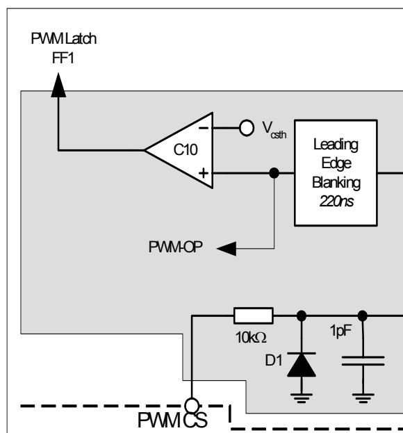
Figure 24 Current Limiting
