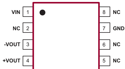
8-lead SOIC (Top view)
