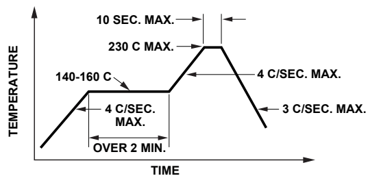
Figure 10. Recommended reflow soldering profile.
