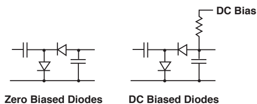
Figure 12. Voltage Doubler.
