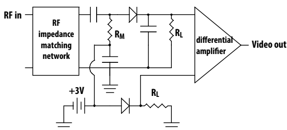
Figure 13. Differential Detector.
