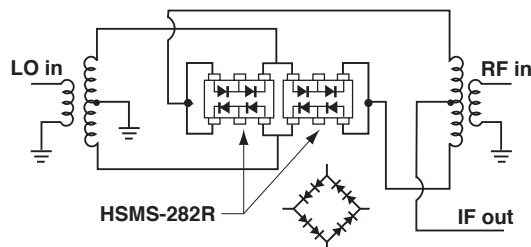
Figure 23. Low Distortion Double Balanced Mixer.
