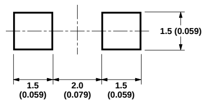
Figure 16. Recommended soldering pattern for HSMx-C150.
