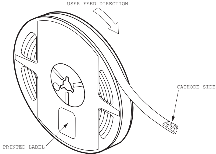
Figure 14. Reeling orientation.
