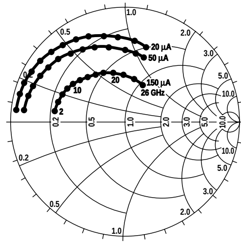
Figure 5. Typical admittance characteristics with external bias. HSCH-5340.
