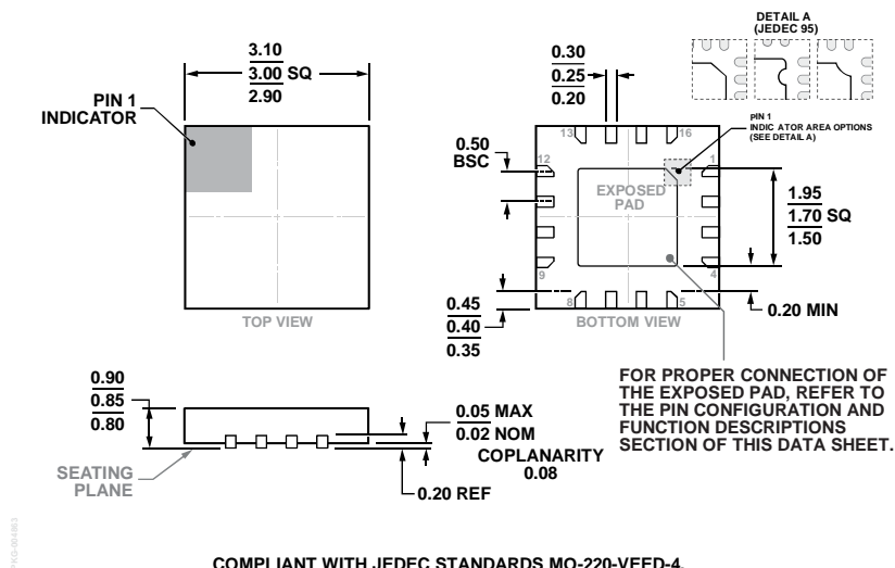
Figure 25. 16-Lead Lead Frame Chip Scale Package [LFCSP] 3 mm × 3 mm Body and 0.85 mm Package Height (HCP-16-1)
