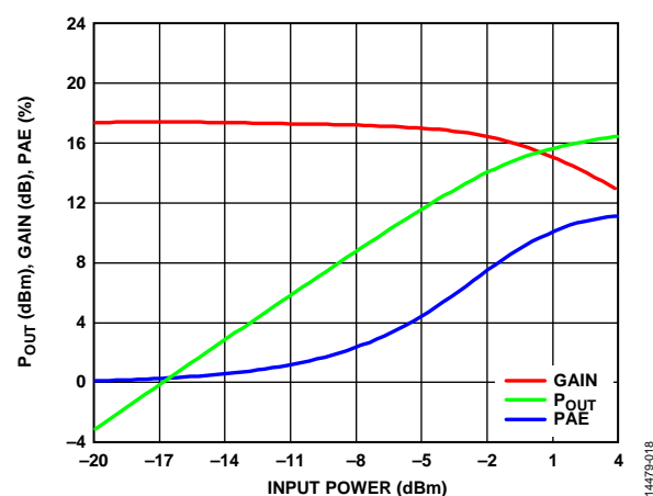
Figure 18. Output Power ( P_{OUT} ), Gain, and Power Added Efficiency (PAE) vs. Input Power (Board Loss Removed from Gain, Power, and Noise Figure Measurements)
