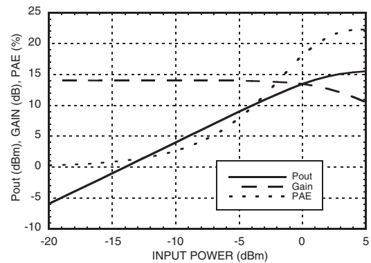
Power Compression @ 5900 MHz [2]
