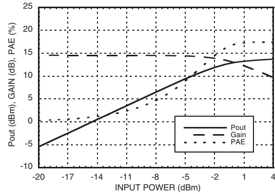
Power Compression @ 4800 MHz [2]
