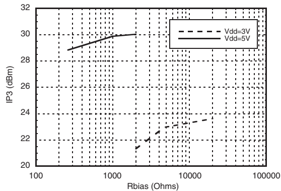
Output IP3 vs. Rbias @ 4800 MHz
