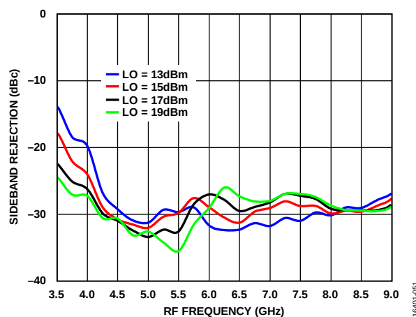
Figure 47. Sideband Rejection vs. RF Frequency at Various LO Power Levels, T_A = 25^\circ\text{C}
