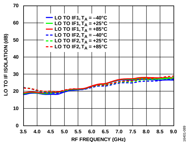
Figure 81. LO to IF Isolation vs. RF Frequency at Various Temperatures, LO = 15 dBm
