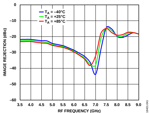
Figure 40. Image Rejection vs. RF Frequency at Various Temperatures, LO = 15 dBm
