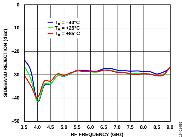
Figure 53. Sideband Rejection vs. RF Frequency at Various Temperatures, LO = 15 dBm
