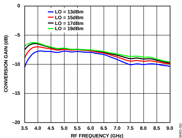
Figure 11. Conversion Gain vs. RF Frequency at Various LO Power Levels, T_A = 25^\circ\text{C}
