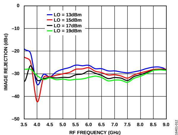
Figure 12. Image Rejection vs. RF Frequency at Various LO Power Levels, T_A = 25^\circ\text{C}
