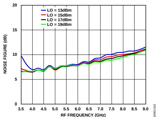
Figure 13. Noise Figure vs. RF Frequency at Various LO Power Levels, T_A = 25^\circ\text{C}
