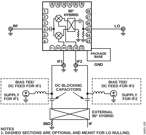
Figure 101. Typical Application Circuit
