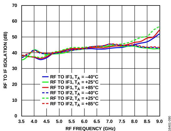
Figure 82. RF to IF Isolation vs. RF Frequency at Various Temperatures, LO = 15 dBm
