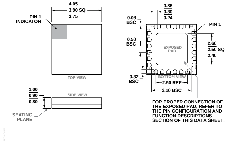
Figure 88. 24-Terminal Ceramic Leadless Chip Carrier [LCC] (E-24-1) Dimensions shown in millimeters
