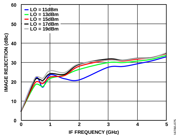
Figure 80. Image Rejection vs. IF Frequency at Various LO Power Levels, T_A = 25^\circ\text{C}
