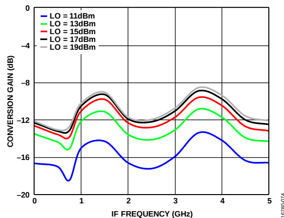
Figure 79. Conversion Gain vs. IF Frequency at Various LO Power Levels, T_A = 25^\circ\text{C}
