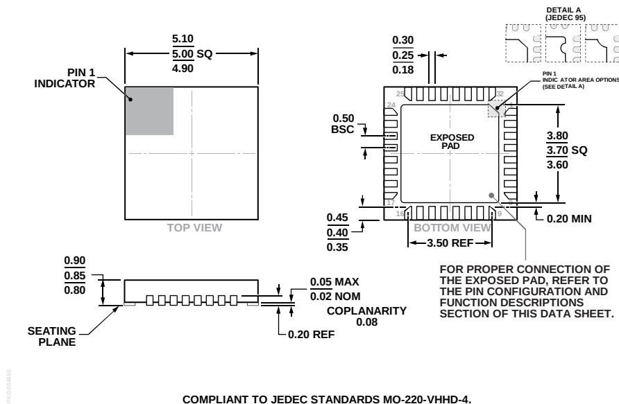
Figure 18. 32-Lead Lead Frame Chip Scale Package [LFCSP] 5 mm x 5 mm Body and 0.85 mm Package Height (HCP-32-1) Dimensions shown in millimeters
