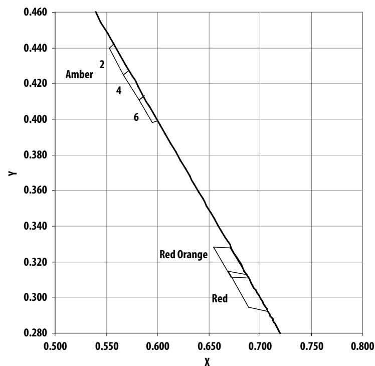
Avago Color Bin on CIE 1931 Chromaticity Diagram
