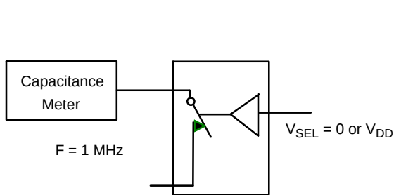
Figure 18. Channel On Capacitance
