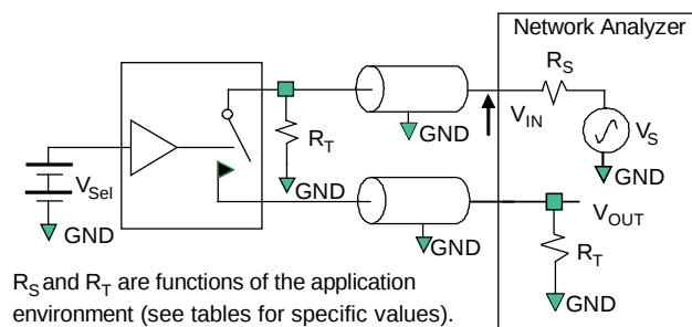
Figure 17. Channel Off Isolation
