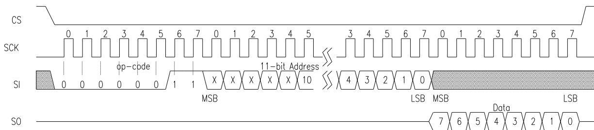
Figure 10. Memory Read
