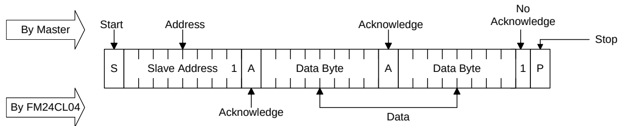
Figure 8. Sequential Read
