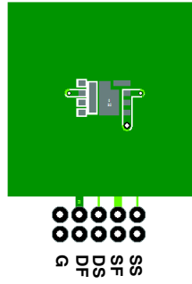
b) 55°C/W when mounted on a 1 in² pad of 2 oz copper.
