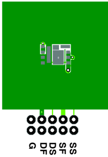
a) 60°C/W when mounted on a 1 in² pad of 2 oz copper.
