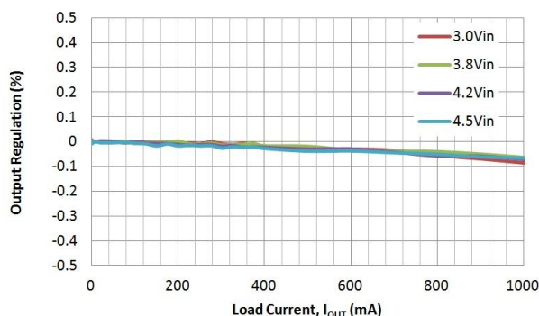
Figure 11. Output Regulation vs. Load Current and Input Voltage
