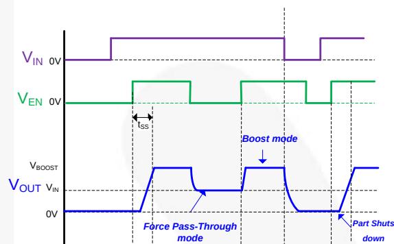
Figure 19. Pass-Through Profile
