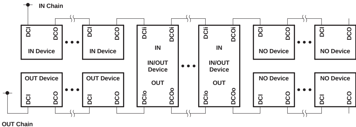
Figure 52. Daisy-Chain Connection
