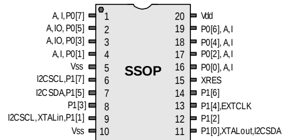
CY8C24223A 20-Pin PSoC Device
