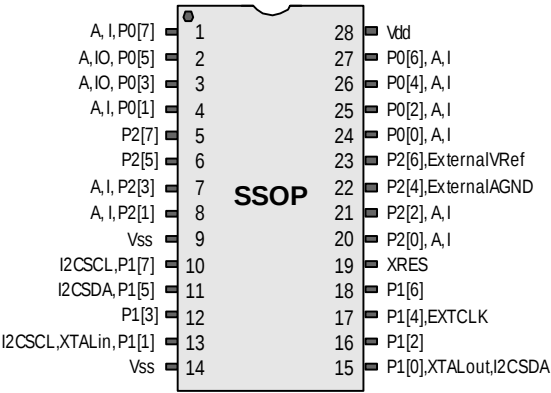
CY8C24423A 28-Pin PSoC Device
