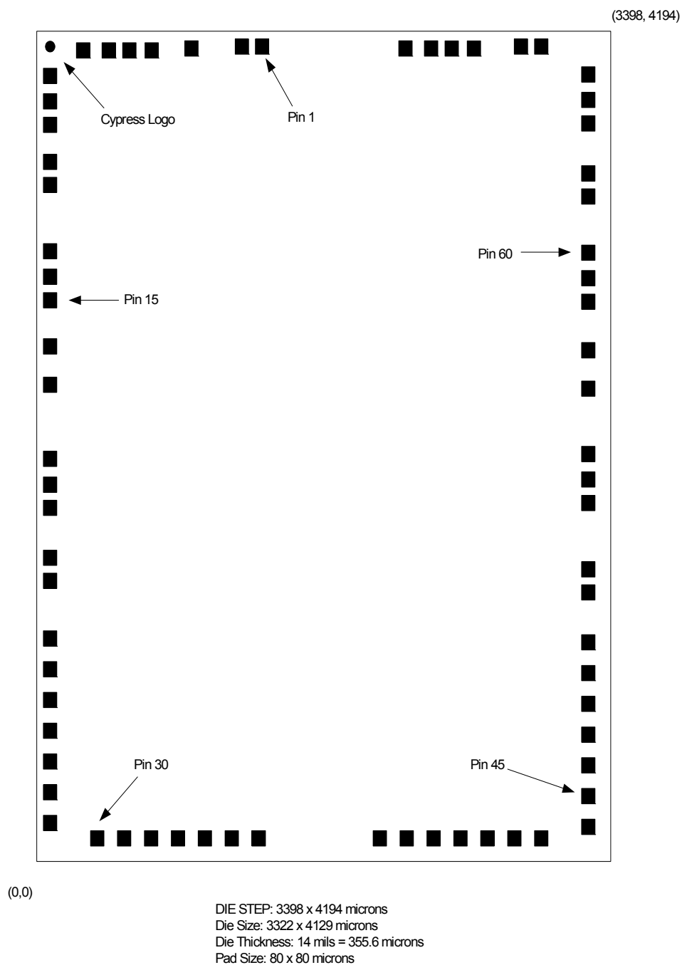
Figure 3. CY7C66113C DIE
