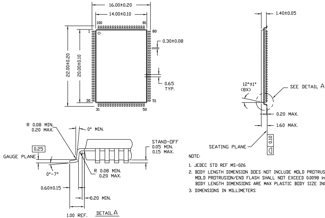
Figure 8. 100-pin Thin Plastic Quad Flatpack (14 × 20 × 1.4 mm), 51-85050
