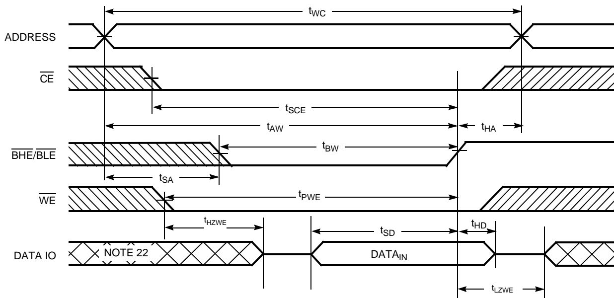
Figure 10. Write Cycle 4: \overline{\text{BHE/BLE}} Controlled, \overline{\text{OE}} LOW [21]
