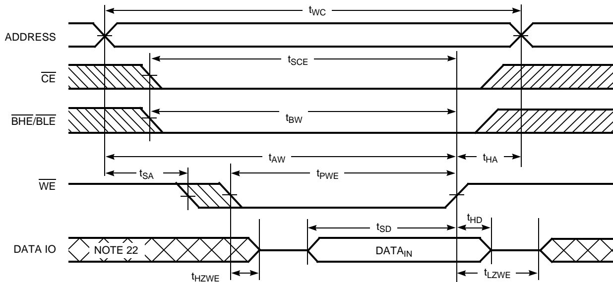
Figure 10. Write Cycle 4: \overline{\text{BHE/BLE}} Controlled, \overline{\text{OE}} LOW [21]
