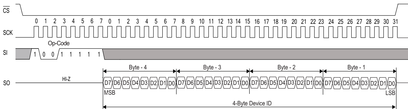
Figure 27. RDID Instruction
