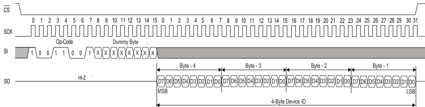
Figure 28. FAST_RDID Instruction
