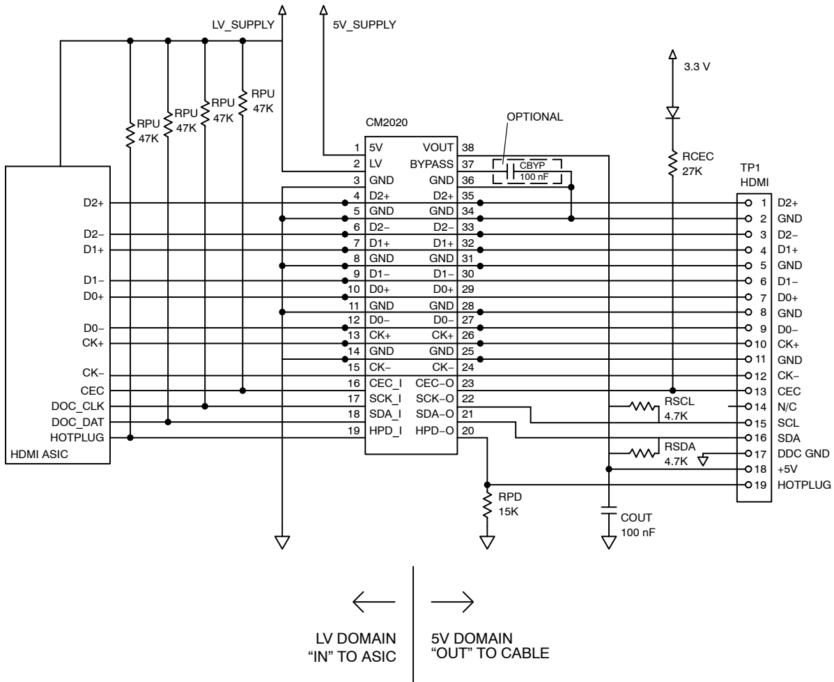
Figure 4. Design Example
