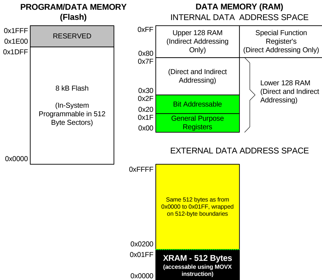
Figure 1.6. Memory Map
