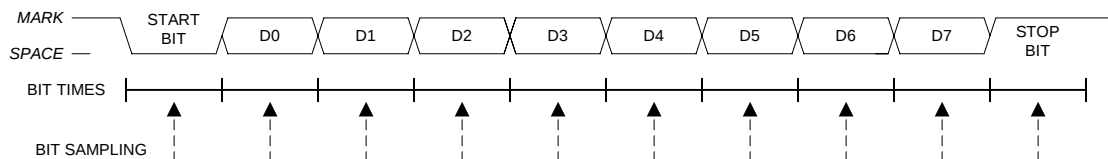
Figure 20.4. 8-Bit UART Timing Diagram
