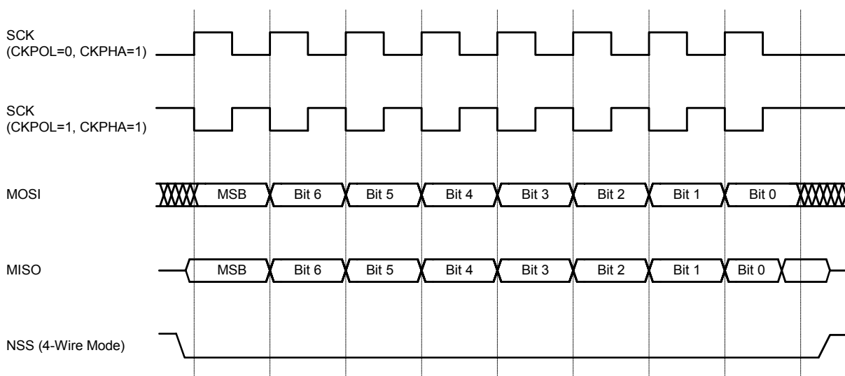
Figure 17.7. Slave Mode Data/Clock Timing (CKPHA = 1)
