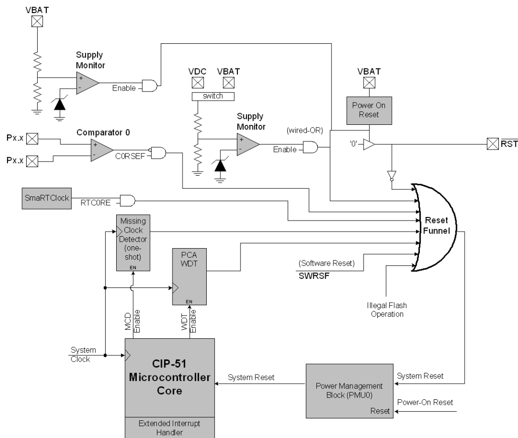
Figure 22.1. Reset Sources
