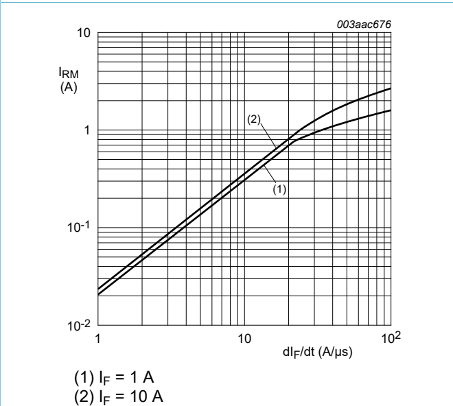
(1) I_F = 1\text{ A} (2) I_F = 10\text{ A} Fig. 9. Peak reverse recovery current as a function of rate of change of forward current and initial forward current; maximum values
