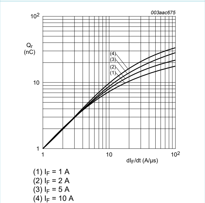
(1) I_F = 1\text{ A} (2) I_F = 2\text{ A} (3) I_F = 5\text{ A} (4) I_F = 10\text{ A} Fig. 10. Recovered charge as a function of rate of change of forward current; maximum values
