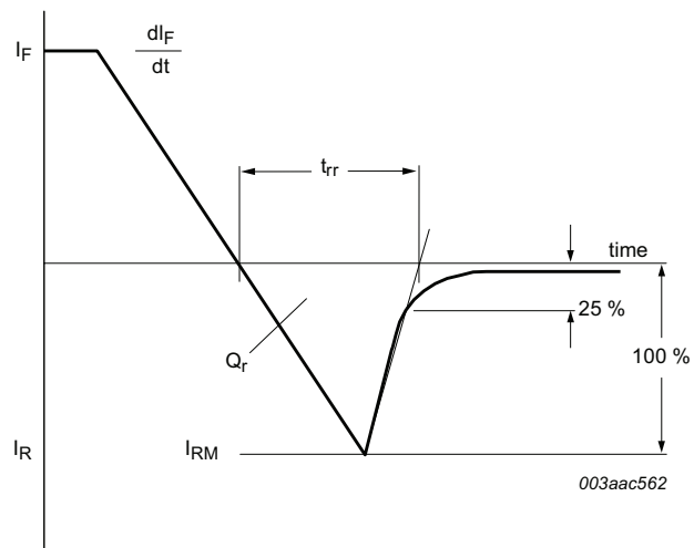
Fig. 5. Reverse recovery definitions; ramp recovery
