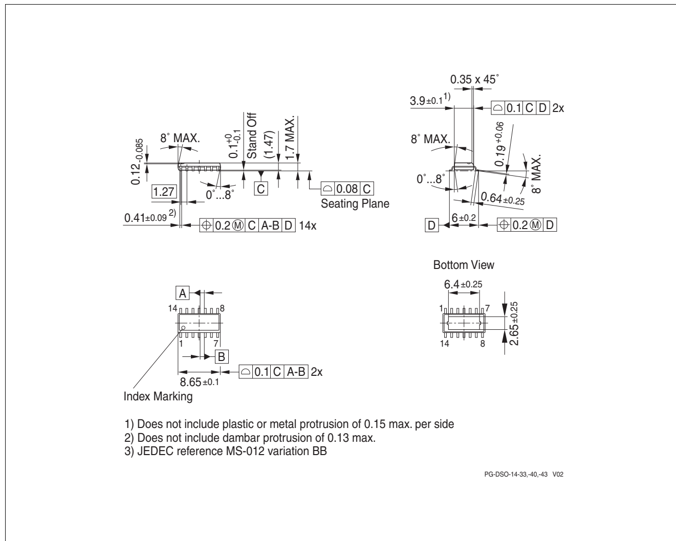
Figure 54 PG-DSO-14-40 EP (Plastic Dual Small Outline Package) (RoHS-Compliant)
