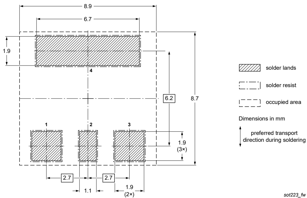
Fig. 18. Wave soldering footprint for SC-73 (SOT223)
