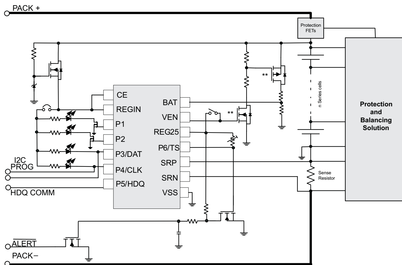
Figure 2. bq34z100 Typical Implementation
