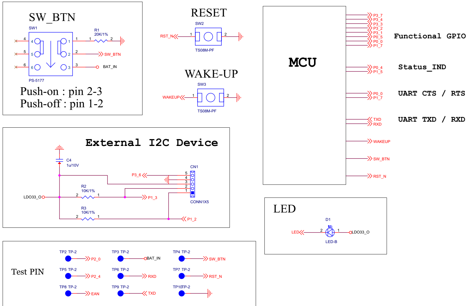
FIGURE 2-10: BM78SPP05MC2/NC2 REFERENCE CIRCUIT
