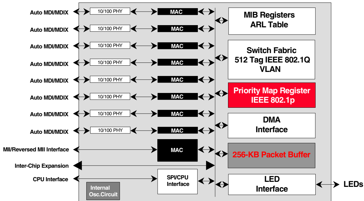
Block Diagram
