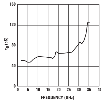
Figure 4. Group Delay.
