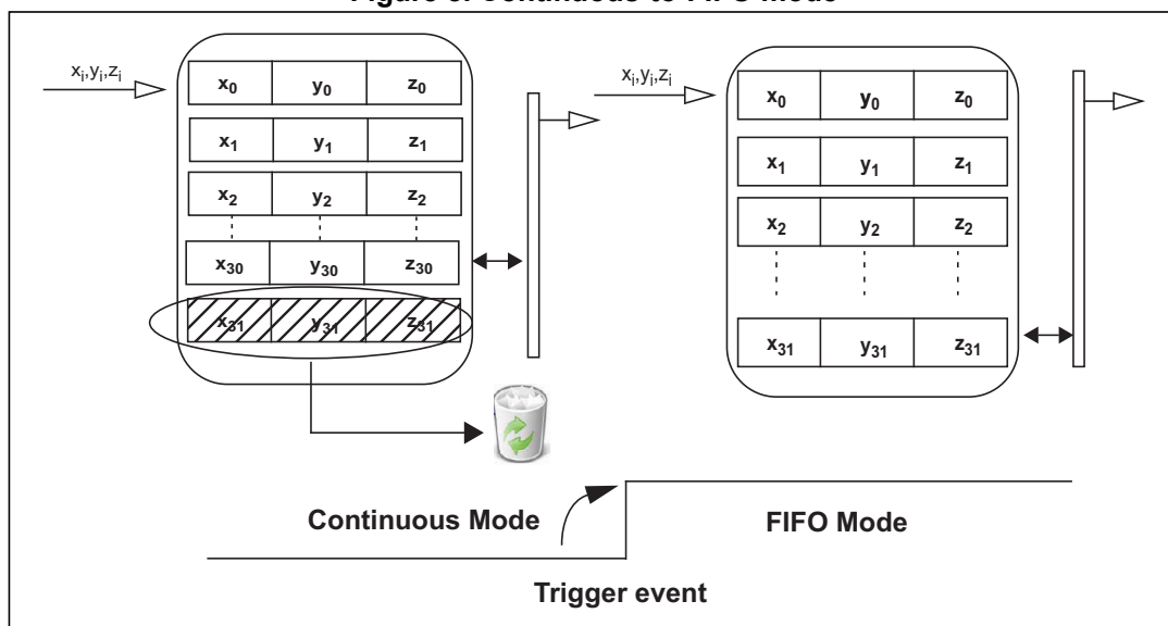
Figure 8. Continuous-to-FIFO mode
