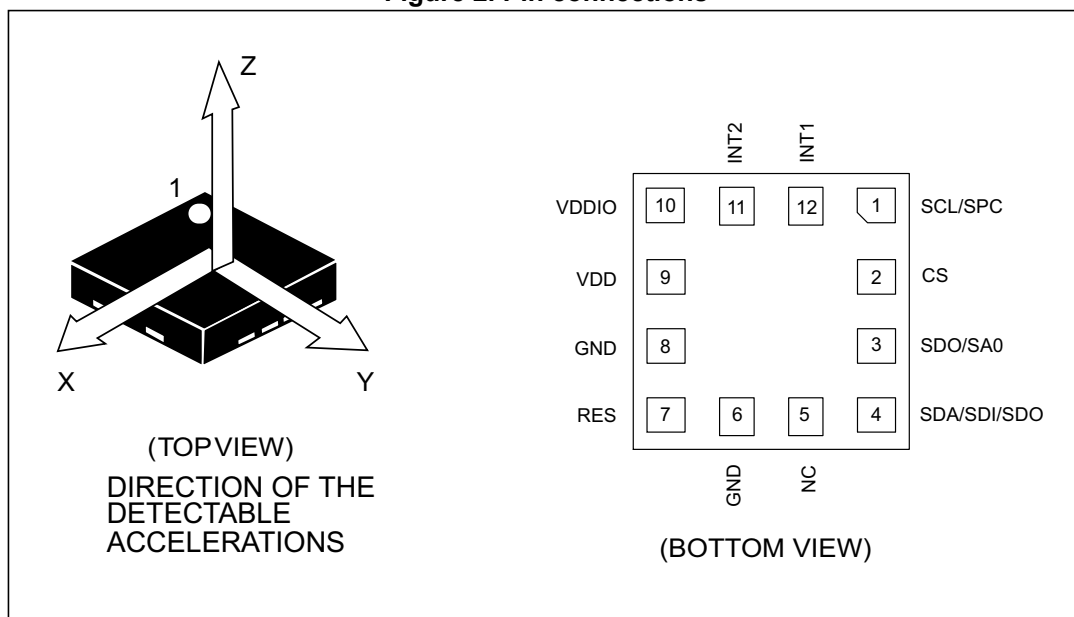
Figure 2. Pin connections
