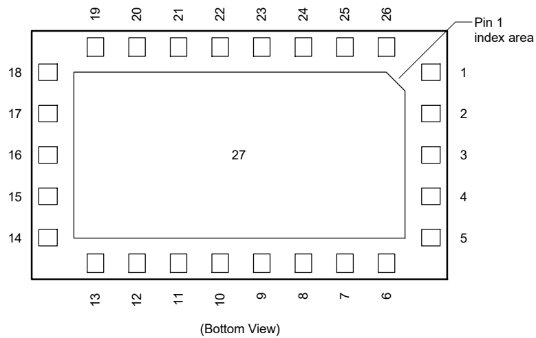
Figure 1. Pin Connections
