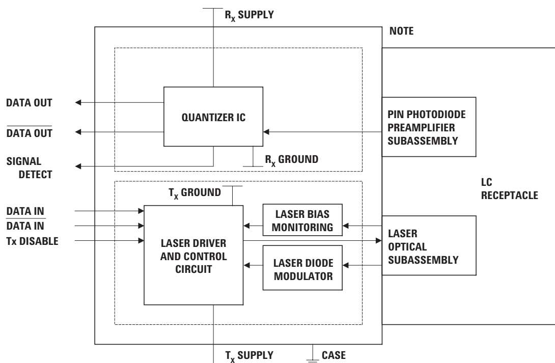
Figure 3. Block Diagram
