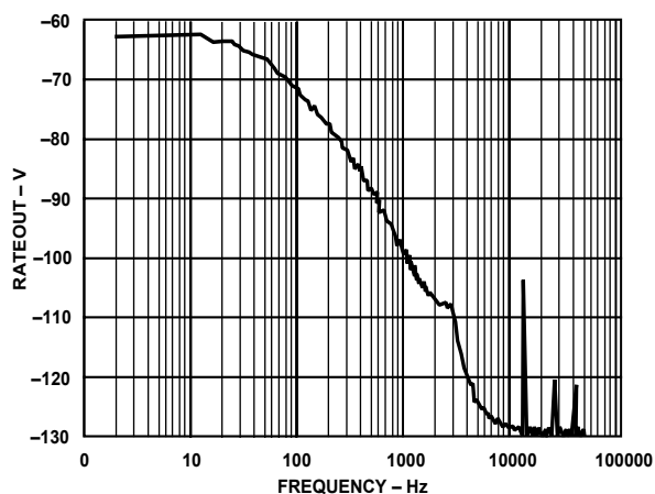
Figure 26. Noise Spectral Density at RATEOUT - BW = 4Hz
