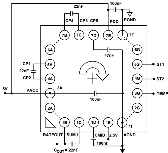
Figure 21. Example Application Circuit (Top View)
