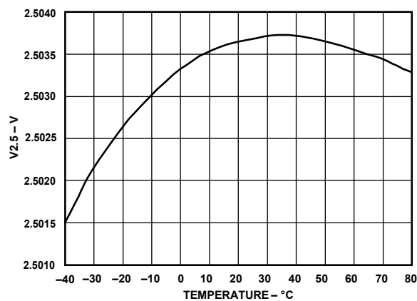
Figure 8. 2.5 V Voltage Reference vs. Temperature
