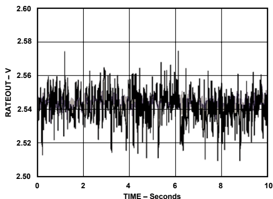
Figure 23. Random Vibration (Lateral) 10 kHz to 20 kHz at 0.01 \text{ g}/\sqrt{\text{Hz}} with 60 Hz Sampling and 0.5 Sec Averaging
