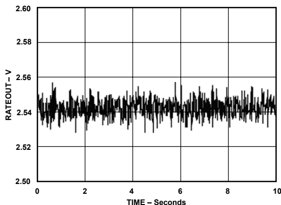
Figure 24. Random Vibration (Lateral) 2 Hz to 40 Hz, 3.2 g rms
