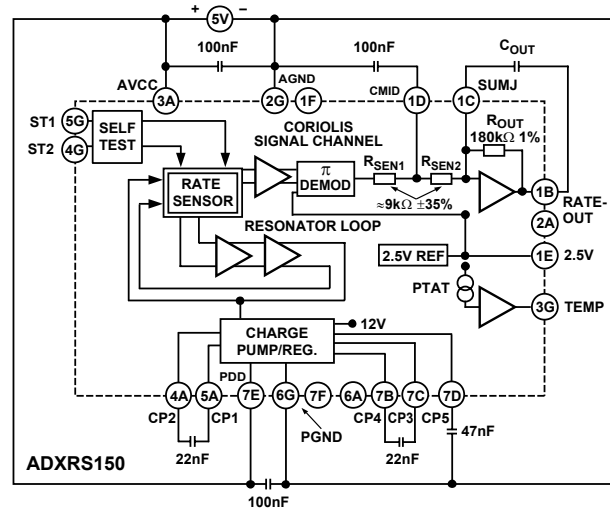
Figure 22. Block Diagram with External Components
