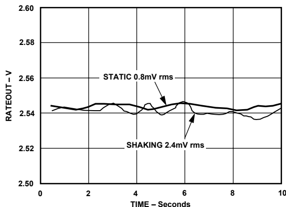
Figure 25. Random Vibration (Lateral) 10 kHz to 20 kHz at 0.01 \text{ g}/\sqrt{\text{Hz}} with 60 Hz Sampling and 0.5 Sec Averaging
