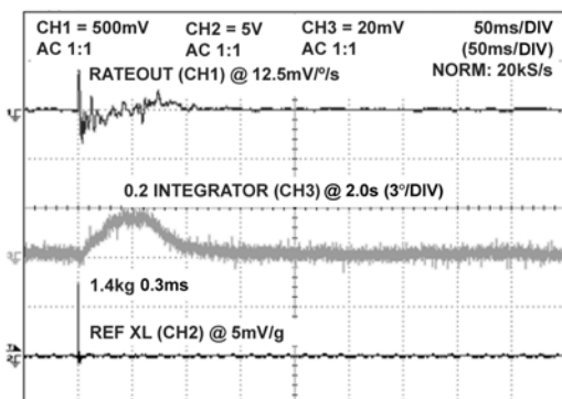
Figure 17. Hi-g Shock in Rate Axis (40 Hz)
