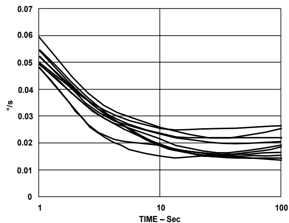
Figure 7. Root Allan Variance vs. Averaging Time
