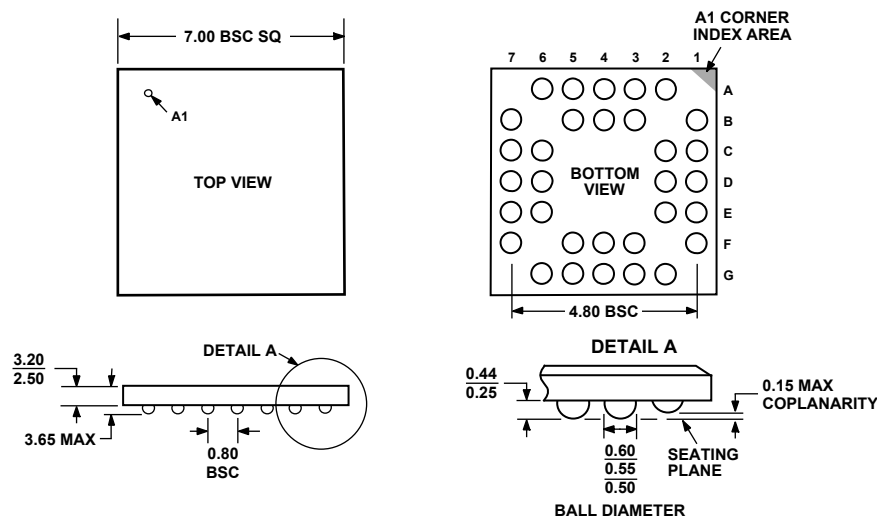
Figure 28. 32-Lead Chip Scale Ball Grid Array [CSPBGA] (BC-32) Dimensions shown in millimeters
