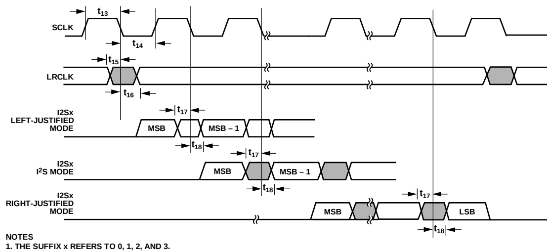
Figure 4. I²S Timing
