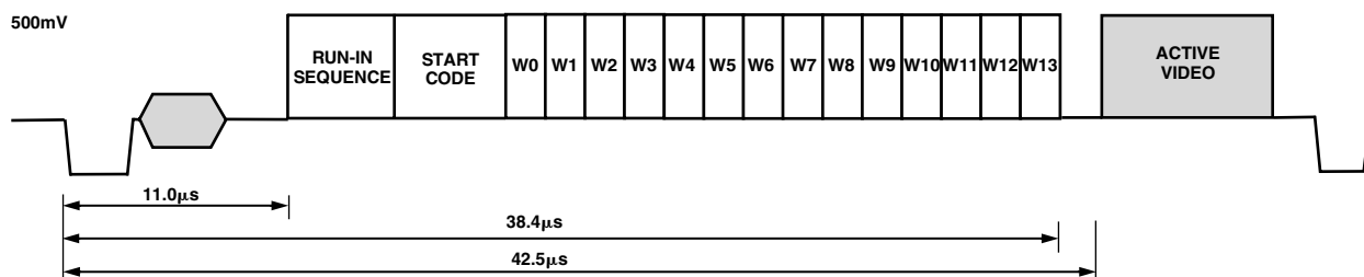
Figure 82. WSS Waveform
