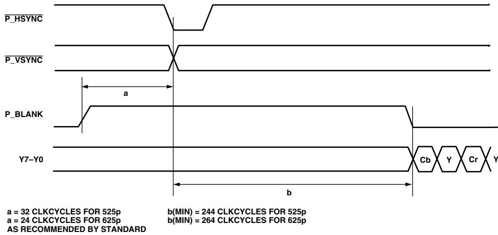
Figure 11. PS 4:2:2 1 x 8-Bit Interleaved @ 54 MHz Input Timing Diagram
