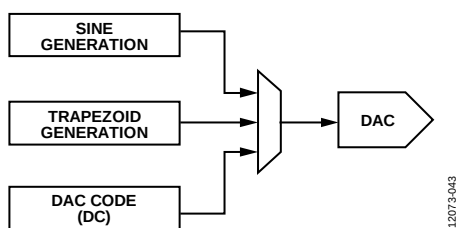
Figure 43. Waveform Generation
