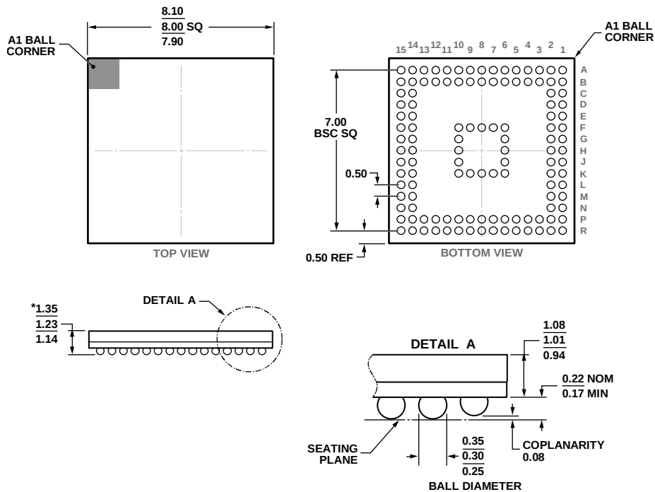
*COMPLIANT TO JEDEC STANDARDS MO-275-CCCE-1 WITH EXCEPTION TO PACKAGE HEIGHT. Figure 45. 120-Ball Chip Scale Package Ball Grid Array [CSP_BGA] (BC-120-3) Dimensions shown in millimeters
