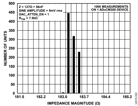
Figure 31. Impedance Measurement Magnitude Precision
