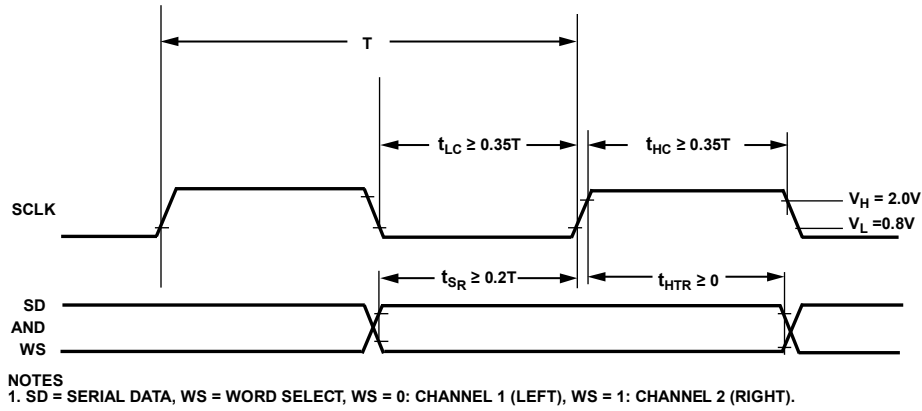
Figure 4. I²S-Compatible Interface Receiver Timing
