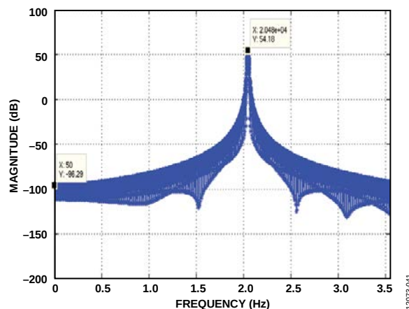
Figure 40. Frequency Response, 2048-Point DFT at 20 kHz
