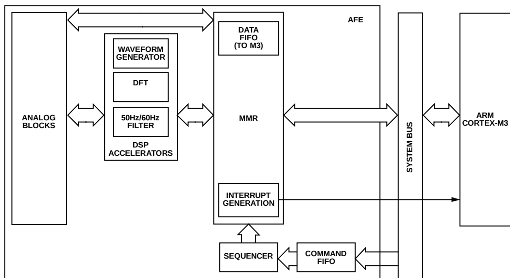
Figure 42. AFE Control
