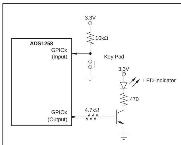
Figure 66. GPIO Connections
