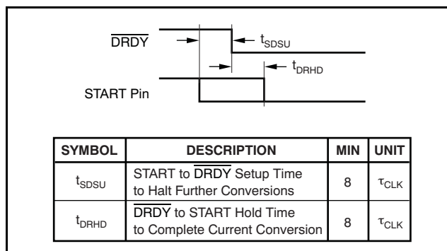
Figure 55. START Pin and DRDY Timing
