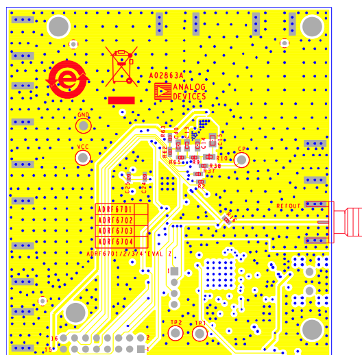
Figure 54. Evaluation Board Bottom Layer
