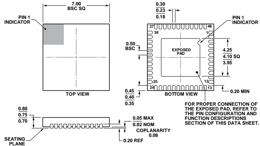
COMPLIANT TO JEDEC STANDARDS MO-220-WKGD. Figure 51. 48-Lead Lead Frame Chip Scale Package [LFCSP] 7 mm × 7 mm Body and 0.75 mm Package Height (CP-48-5) Dimensions shown in millimeters
