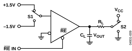
Figure 9. Receiver Enable/Disable
