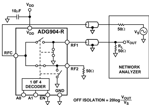
Figure 20. Off Isolation
